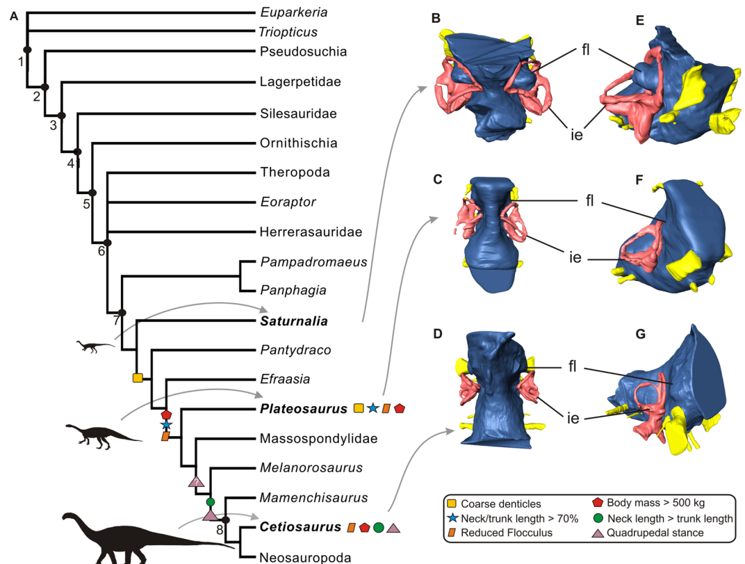
Figure 2. Simplified Archosauriformes phylogeny highlighting character acquisition in Saupodomorpha (A). Endocasts of Saturnalia tupiniquim (MCP-3845-PV), Plateosaurus (MB.R.5586-1), and a saupod specimen tentatively referred to Cetiosaurus (OUMNH J13596) in dorsal (B,C,D) and anterolateral (E,F,G) views showing the morphology of the Floccular Fossae Lobe in saupodomorph dinosaurs. Abbreviations: fl – Floccular Fossae Lobe, ie – inner ear, 1 – Archosauriformes, 2 – Archosauria, 3 – Dinosauriformes, 4 – Dinosauria, 5 – Saurischia, 6 – Saurischia, 7 – Saupodomorpha, 8 – Sauropoda.
