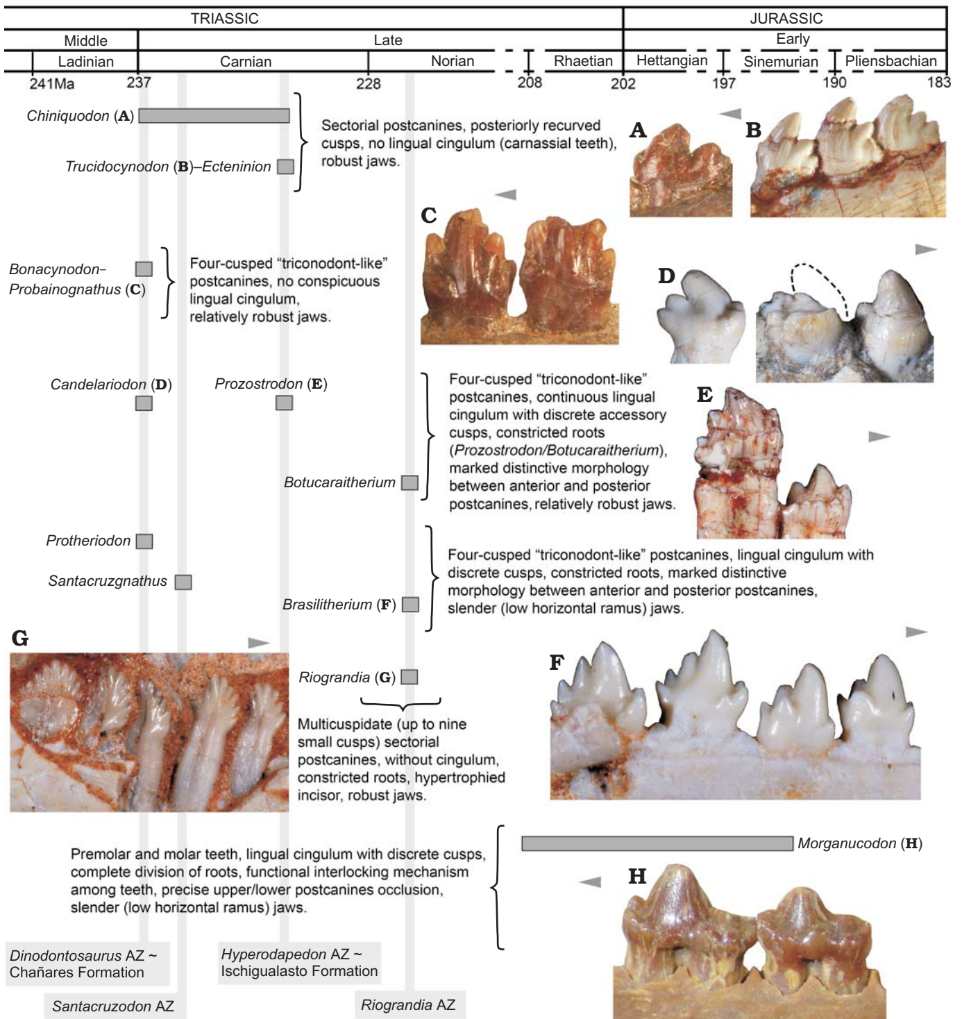
Fig. 8. Main dental features of selected non-mammaliaform probainognathians and one mammaliaform ( Morganucodon ) disposed in a time scale. A. Chiniquodon thetonicus , PVL 4444, left lower postcanine in labial view. B. Trucidocynodon riograndensis , UFRGS-PV-1051-T, left lower postcanines in labial view. C. Probainognathus jenseni , PVL 4445, right lower pc5–6 in lingual view. D. Candelariodon barberenai , MMACR PV-0001-T, left lower postcanines in lingual view. E. Prozostrodon brasiliensis , UFRGS-PV-0248-T, left lower postcanines in labial view. F. Brasilitherium quadrangularis , UFRGS-PV-0603-T, left lower postcanines in labial view. G. Riograndia guaibensis , UFRGS-PV-0833-T, left lower postcanines in lingual view. H. Morganucodon watsoni , NHMUK-PV-M-U273, right postcanines in lingual view. Arrows indicate mesial side of the dentition.
