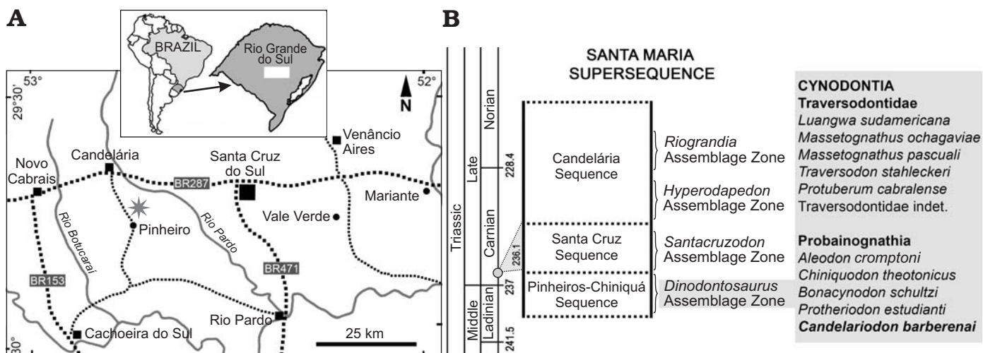
Fig. 1. Geographic (A, star indicates the type locality) and biostratigraphic (B) location of Candelariodon barberenai . The biostratigraphy follows Horn et al. (2014) and the dating (grey circle in B) corresponds to Philipp et al. (2013).
